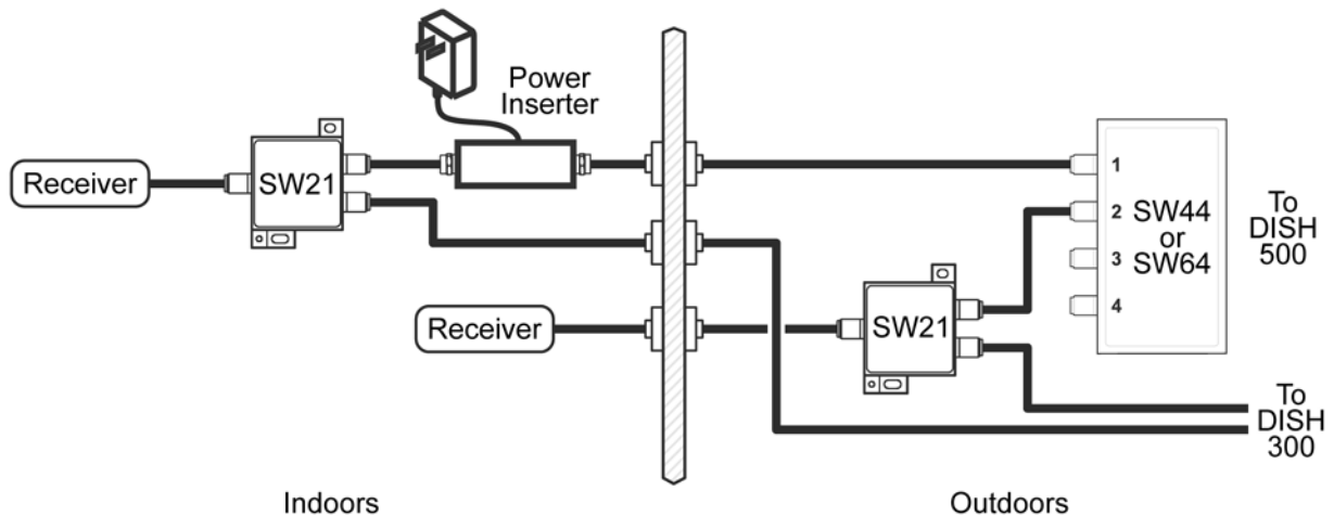
Figure 1 - Installation with Power Inserter and SW21 on the Same Cable
