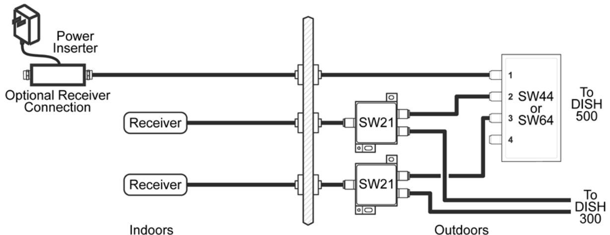
Figure 2 – Alternate Installation Using a Power Inserter on a Dedicated Cable
