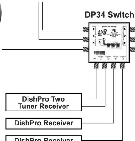
DISH 500 DishPro TWIN or 2 DishPro Single LNBs
